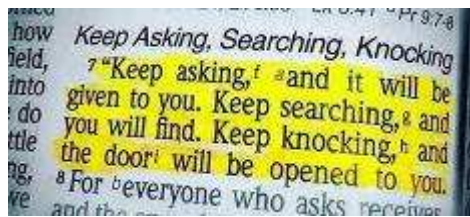
Mt 7.8
